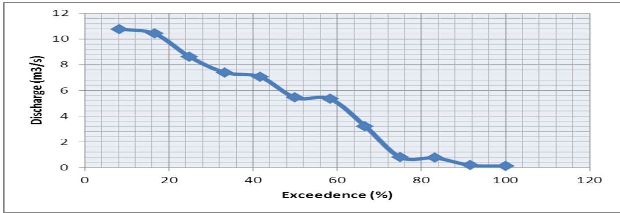
Figure 4. Flow duration curve at Orle river
