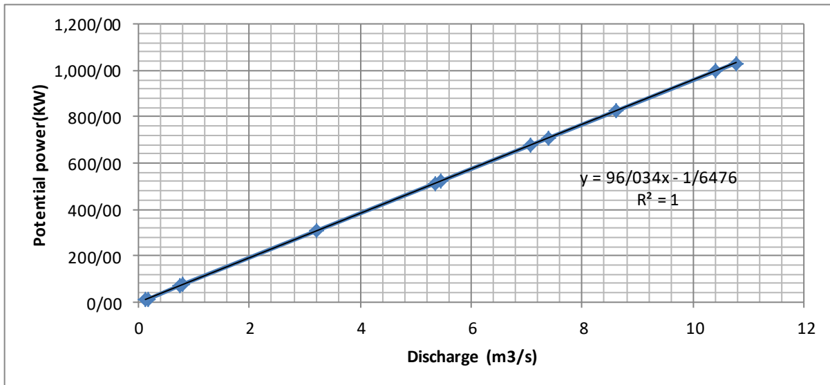
Figure 5. Potential power rating and river discharge
