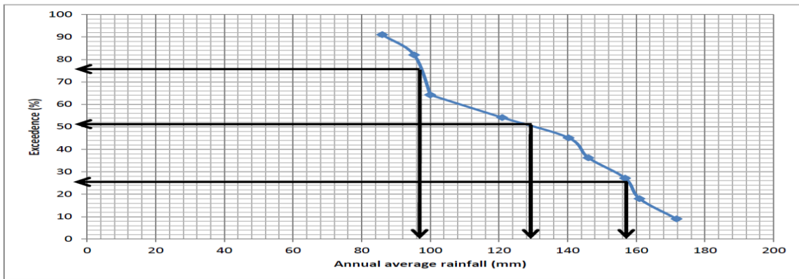
Figure 3. Rainfall frequency-exceedence curve
